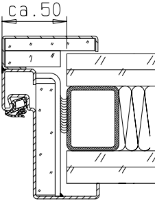
Zarge "ZG 68/76"
