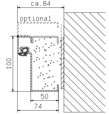
Zarge "ZG 68/76"
