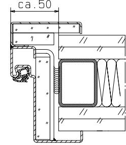
Zarge "ZG 68/76"
